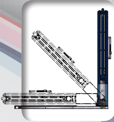
ALBERO RECLINABILE HINGEN MAST
